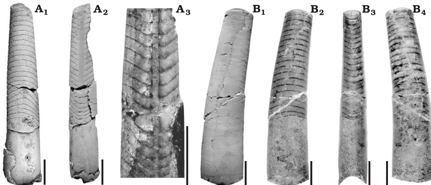
Fig. 10. A. Holotype of Pomerantsoceras pollux “var. castor ” (Barrande, 1866). Specimen NM-L 571, in lateral (A 1 ) and ventral (A 2 ) views, and detail of the siphuncle (A 3 ); Butovice Na Břekvici Section, Colonograptus colonus Zone, Gorstian, Ludlow. B. Holotype of Pomerantsoceras pollux (Barrande, 1866). Specimen NM-L 570, in lateral view showing diagenetic rupture of the shell (B 1 ); and lateral (B 2 , B 4 ) and ventral (B 3 ) views. Malá Chuchle, Vyskočilka locality, Testograptus testis , Homesian, Wenlock. Specimens A 1 , A 2 , and B 1 are coated with ammonium chloride. Scale bars 5 mm.
