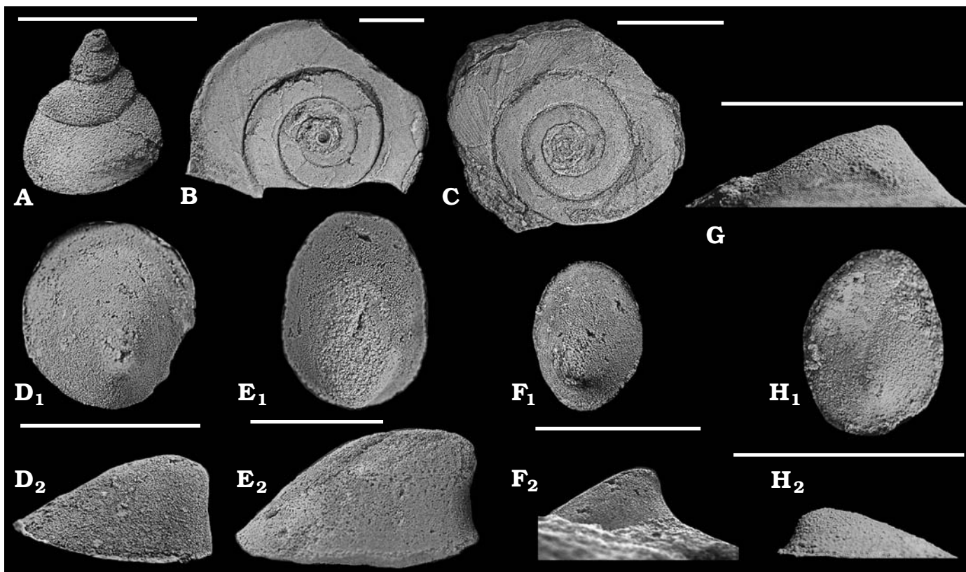
Fig. 13. Gastropods from the Stairway Sandstone, Middle Ordovician, Australia. All internal moulds. A. Raphistomina? sp. from Areyonga Gorge with 4 whorls (CPC 41496). B, C. Teiichispira? sp. from loose samples from Petermann Creek; with a very flat base, perhaps 5 whorls present ( B. CPC 41497; C. CPC 41498). D, E. Archinacelloid sp. A ( D. CPC 41499; E. CPC 41500) from Petermann Creek; with slightly concave subapical surface and steeply inclined slightly curved apex, in anterior ( D 1 , E 1 ) and left-lateral ( D 2 , E 2 ) views. F, G. Archinacelloid sp. B from Areyonga Gorge ( F ) and Petermann Creek ( G ). F. Specimen with subcentral and sharply pointed apex (CPC 41501), in anterior ( F 1 ) and left-lateral ( F 2 ) views. G. Specimen with subcentral and pointy apex (CPC 41502), in left-lateral view. H. Archinacelloid sp. C from Petermann Creek with low shell profile and inclined slightly curved apex (CPC 41503), in anterior ( H 1 ) and left-lateral ( H 2 ) views. Scale bar 10 mm.
