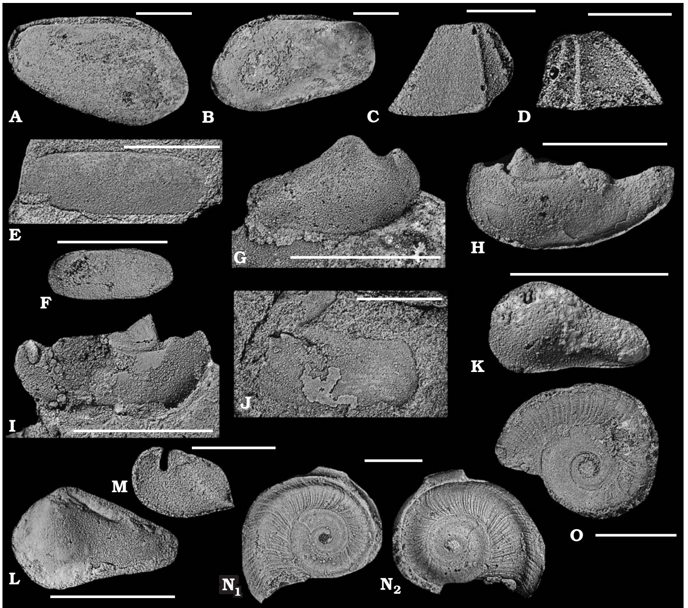
Fig. 12. Pteriormorphian and heteroconchian bivalves, rostroconchs and gastropods from the Stairway Sandstone, Middle Ordovician, Australia. Internal moulds (A, B, E–M, N 1 ) and latex casts of internal (N 2 , O) and external (C, D) moulds. A, B. Modiolopsis pojetai sp. nov. from Petermann Creek. A. Holotype (CPC 41481) in left-lateral view showing discrete longitudinal dorsal slit-like mark. B. Paratype (CPC 41482) in right-lateral view with umbo steeply descending anteriorly. C, D. Colpantyx? sp. A from Areyonga Gorge; in right (C, CPC 41483) and left-lateral (D, CPC 41484) views with two umbonal radial ribs anteriorly and one posteriorly. E, F. Sphenosolen draperi Pojeta and Gilbert-Tomlinson, 1977 from Petermann Creek ( E , CPC 41485; F , CPC 41486), specimens with flat shell and narrow elongated sub-rectangular shape. G–M. Rostroconchia. G–I. Ribeiria csiro Pojeta, Gilbert-Tomlinson, and Shergold, 1977 from Areyonga Gorge (G) and Petermann Creek (H–I); note the prominent triangular beak and curved ventral margin ( G , CPC 41487; H , CPC 41488; I , CPC 41489). J. Ribeiria jonesi? from Petermann Creek, sub-rectangular profile and strong dorsally projecting umbo (CPC 41490). K, L. Pinnocaris sp. A from Petermann Creek with inflated pear-shaped profile ( K , CPC 41491; L , CPC 41492). M. Technophorus walteri Pojeta, Gilbert-Tomlinson, and Shergold, 1977 from Areyonga Gorge (CPC 41493) with a single lateral radial rib and prominent nearly erect pegma indicated. N, O. Gastropoda, Scalites? sp. from Petermann Creek. N. CPC 41494 (N 1 ), latex cast with clear growth lines (N 2 ). O. CPC 41495, specimen with 3.5 to 4 whorls. Scale bars 10 mm, except C, D, M, 5 mm.
