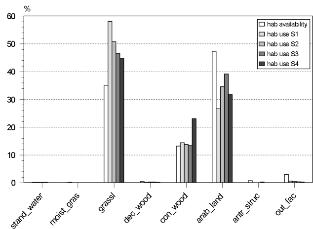
Fig. 2. Availability in the study area (%) and use (%), mean value of radio tracked individuals) of eight habitat categories within home ranges (K95) of raccoon dogs during four seasons (S1: February to April, S2: May to July, S3: August to October, S4: November to January).
