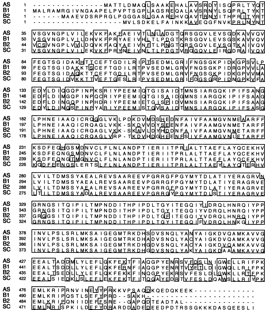
Fig. 4. Alignment of the amino acid sequences of subunit B of V-ATPases from various organisms. Identical residues are boxed. Abbreviations: AS, Ascidia sydneiensis samea (this study); B1, bovine brain-type isoform (Puopolo et al. , 1992); B2, bovine renal-type isoform (Nelson et al. , 1992); SC, budding yeast (Nelson et al. , 1989).
