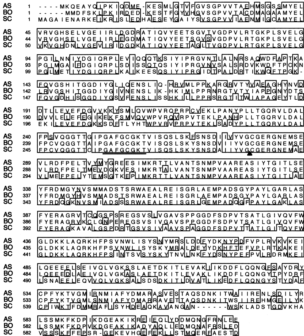
Fig. 2. Alignment of the amino acid sequences of subunit A of V-ATPases from various organisms. Identical residues are boxed. The P-loop motif is underlined. The solid triangle shows the position of protein splicing, which generates a DNA endonuclease (Gimble and Thorner, 1992) in yeast. Abbreviations: AS, Ascidia sydneiensis samea (this study); BO, bovine (Puopolo et al. , 1991); SC, budding yeast (Hirata et al. , 1990).
