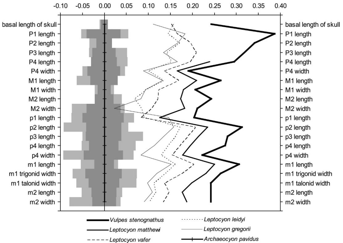
Fig. 17. Log-ratio diagram comparing the means of the cheek tooth dimensions (appendix 3) of four species of Leptocyon with Vulpes stenognathus using the primitive borophagine Archaecocyon pavidus as the standard. Gray bars extending from the mean of the standard are the observed ranges (light) and \pm 1\sigma (dark) of the mean of the sample used.
