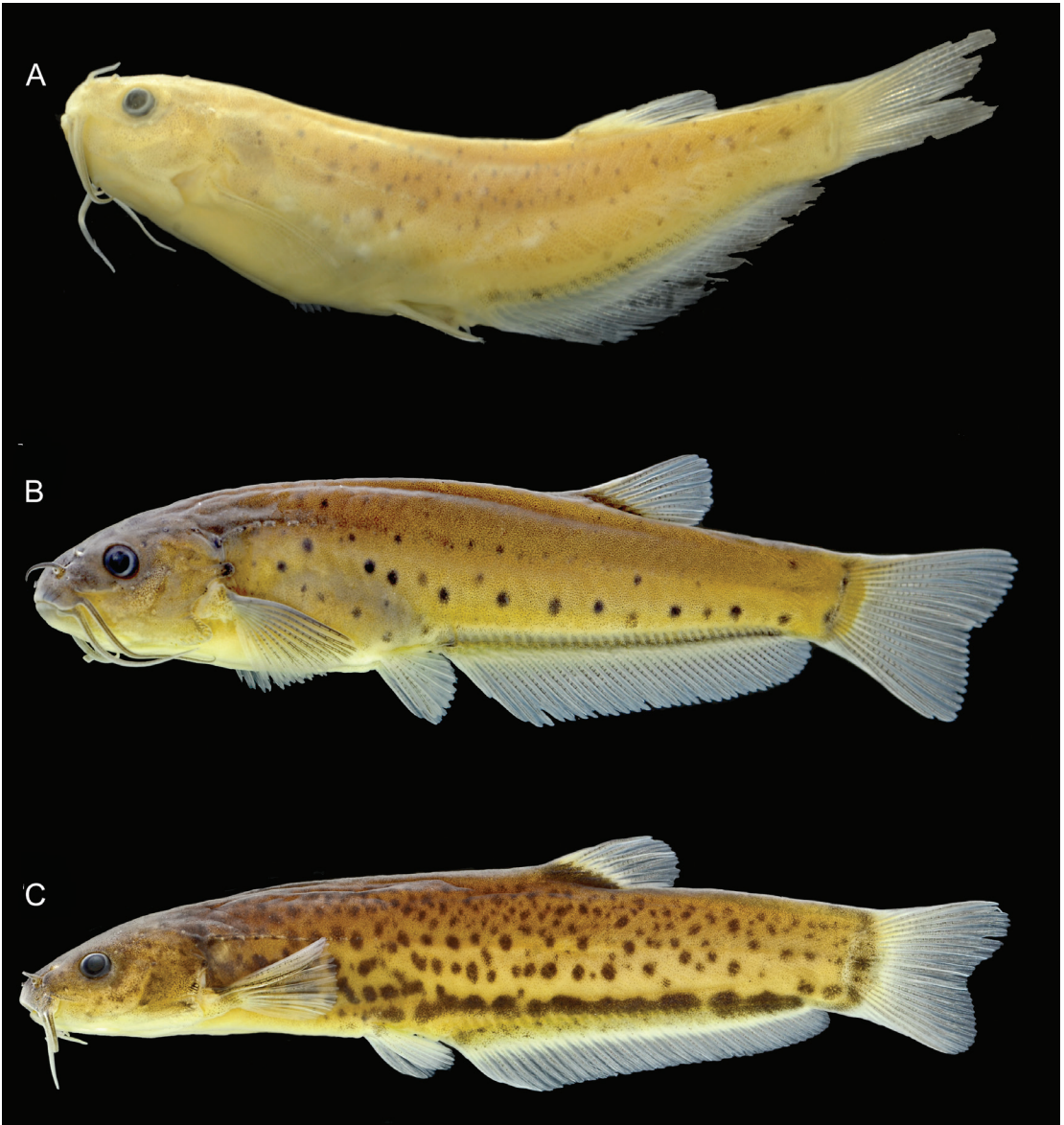
FIG. 2. Comparative illustrations of species of Trichogenes . A. T. beagle , 35.5 mm SL (MZUSP 125019, holotype). B. T. claviger , 47.7 mm SL (MZUSP 124882). C. T. longipinnis , 56.8 mm SL (MZUSP 111153).
