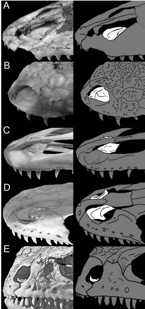
FIGURE 4. Comparisons of snout morphologies in the Anguimorpha, with the septomaxilla highlighted in white. A. Estesia mongoliensis (IGM 3/196); B. Heloderma suspectum (AMNH R-147173); C. Varanus salvadorii (AMNH R-59873); D. Lanthanotus borneensis (the Deep Scaly Project, 2011b); E. Shinisaurus crocodilurus (Bever et al., 2005). Not to scale.
