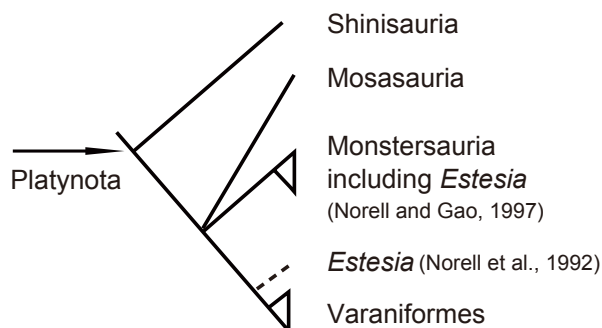
FIGURE 1. Two possible phylogenetic positions for Estesia mongoliensis suggested in previous studies. The cladogram of the Platynota follows Conrad (2008).
