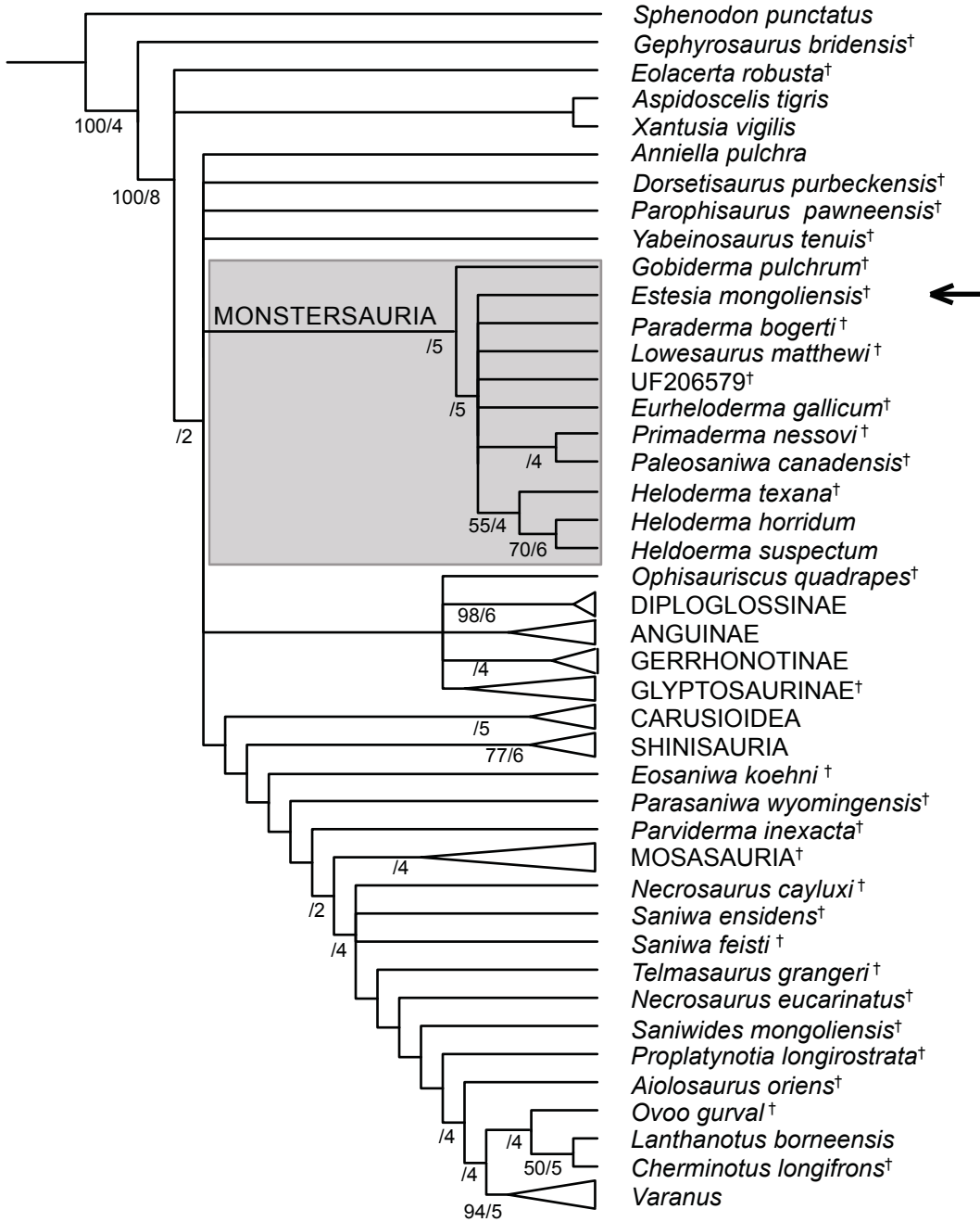
FIGURE 9. The strict consensus tree of the combined analysis of morphological and molecular data. Support values are labeled beneath branches. The number written before the slash is bootstrap value; the number written after the slash is Bremer support. Only bootstrap values above 50% are listed, so some branches show only Bremer support values.
