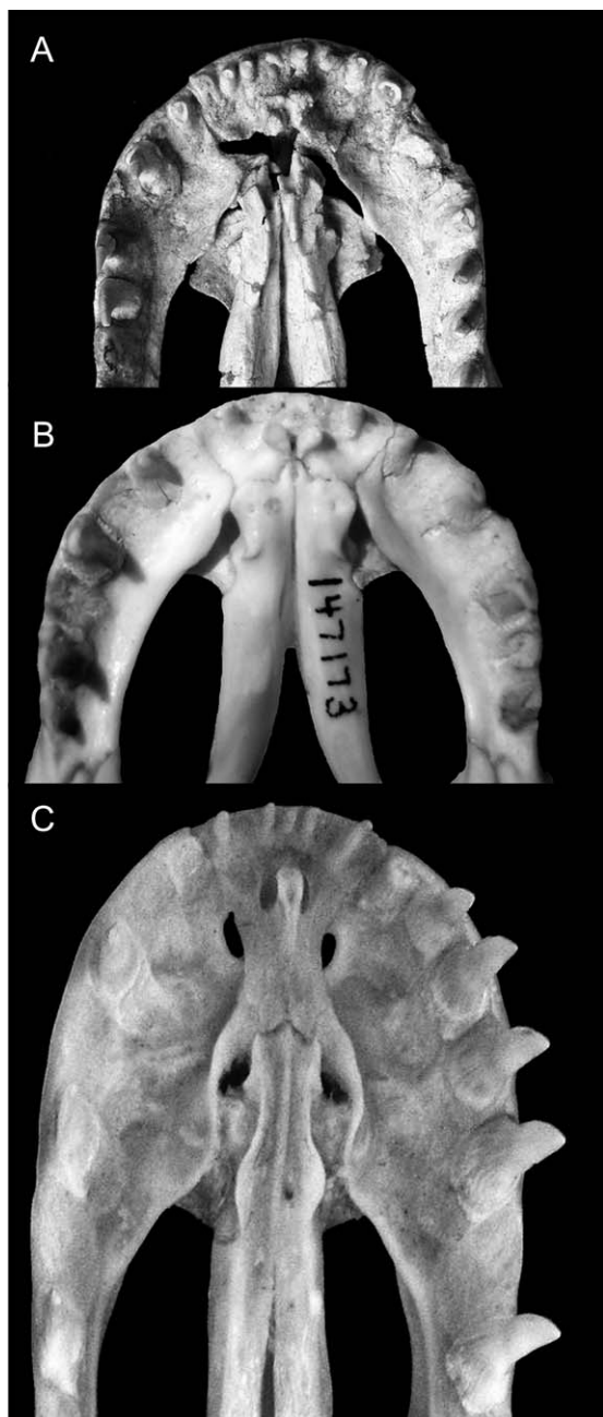
FIGURE 5. Comparisons of anterior palate of: (A) Estesia mongoliensis (IGM 3/196); (B) Heloderma suspectum (AMNH R-147173); and (C) Varanus salvadorii (AMNH R-59873). Not to scale.
