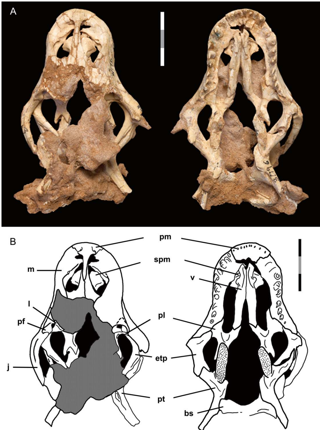
FIGURE 3. A. Skull of IGM 3/196 in dorsal and ventral view (scale bar = 10 mm). B. Line drawings of the skull of IGM 3/196 in dorsal and ventral view (scale bar = 10 mm). Abbreviations are listed in appendix 6.
