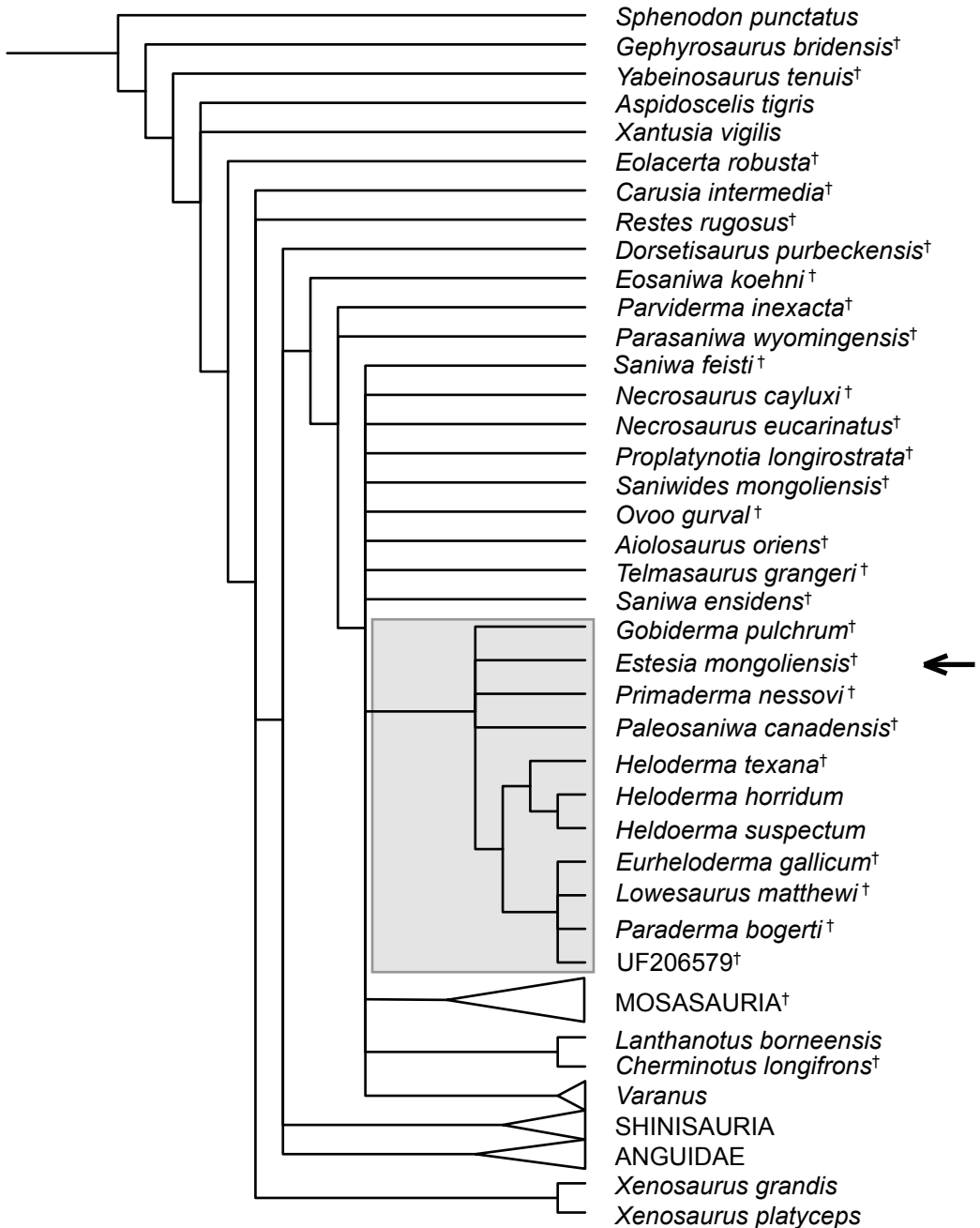
FIGURE 10. The strict consensus tree of the morphology-only analysis. The clade in grey shade is the Monstersauria.
