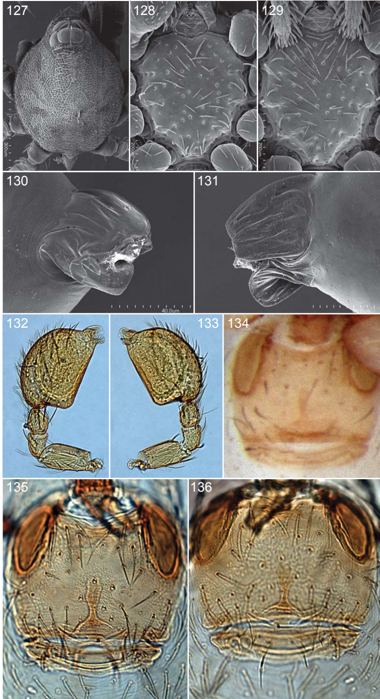
FIGS. 127–136. Scaphioides granpiedra , new species, male (127, 128, 130–133) and female (129, 134–136). 127. Carapace, dorsal view. 128, 129. Sternum, ventral view. 130. Left embolus, proterolateral view. 131. Same, retrolateral view. 132. Left palp, proterolateral view. 133. Same, retrolateral view. 134. Epigastric region, ventral view. 135. Genitalia, ventral view. 136. Same, dorsal view.
