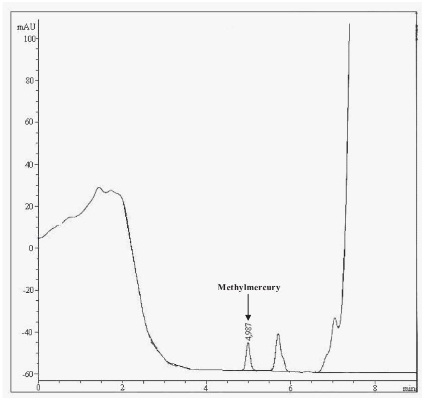
Figure 5. Chromatogram of the locality Frontera Peña—Orinoco contaminated with methylmercury standard of 50 \text{ ng}\cdot\text{ml}^{-1} , in a proportion 1:1. Retention time for MeHg = 4.99 minutes.
