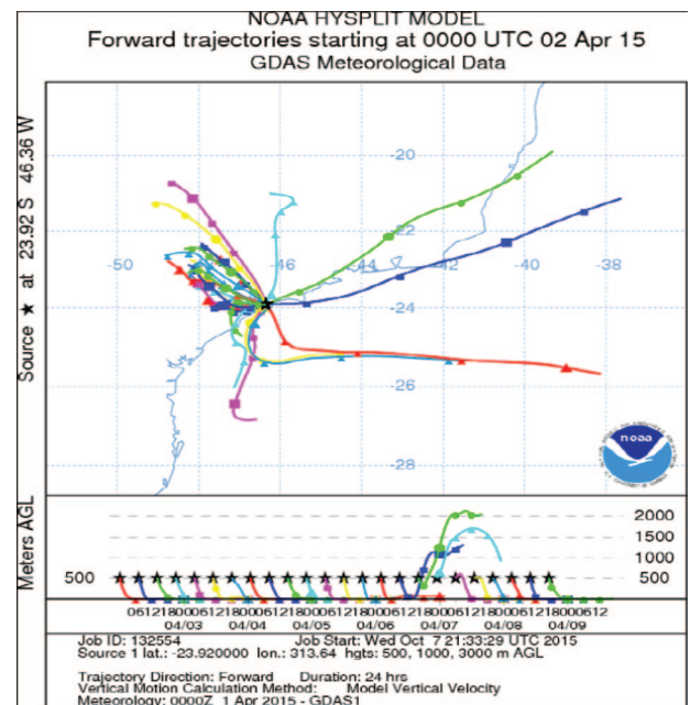
Figure 4. Plumes generated during the days of the fire. Source: HYSPLIT (Hybrid Single-Particle Lagrangian Integrated Trajectory).
