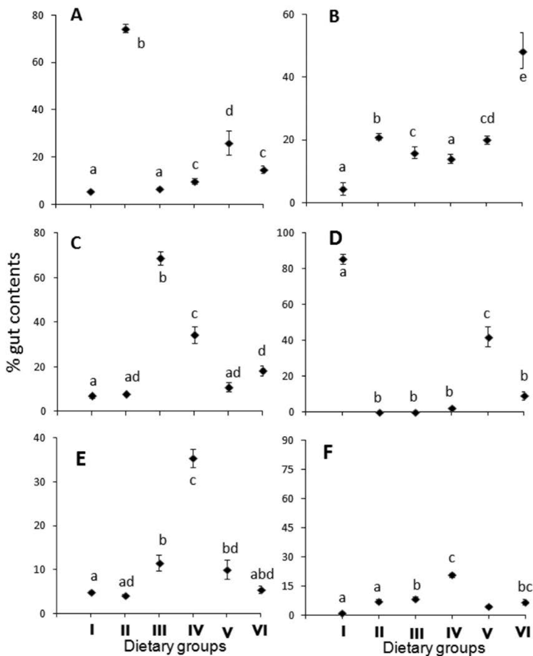
Figure 3. Mean ( \pm 1 SE) percentages of vascular plant material (VPM; >1 mm) (A), coarse particulate organic matter (CPOM; 50 \mu\text{m} - 1 mm) (B), fine particulate organic matter (FPOM; <50 \mu\text{m} ) (C), animal material (AM) (D), algae (ALG) (E), and inorganic matter (IM) (F) in the gut contents of individuals belonging to dietary groups I–VI. Points with the same lowercase letter are not significantly different among dietary groups ( p < 0.05 ). See Fig. 2 for a description of dietary groups.
