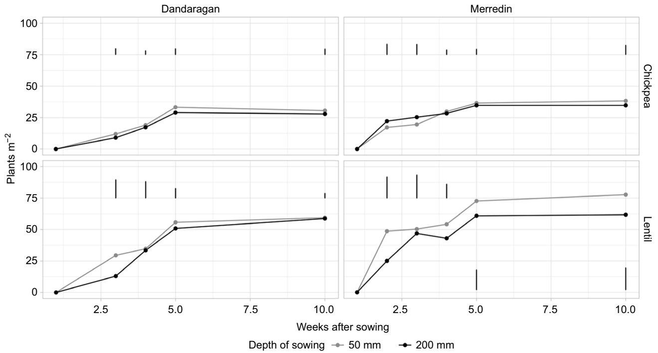
Fig. 6. Emergence of Striker chickpea and Bolt lentil from standard (50 mm) and deep (200 mm) sowing depths over the first 10 weeks after sowing. Counts were taken manually from two sections of 13-m 2 plots sown in May at Dandaragan and Merredin in Western Australia. Vertical lines represent l.s.d. ( P = 0.05 ) values comparing sowing depths at individual count times.
