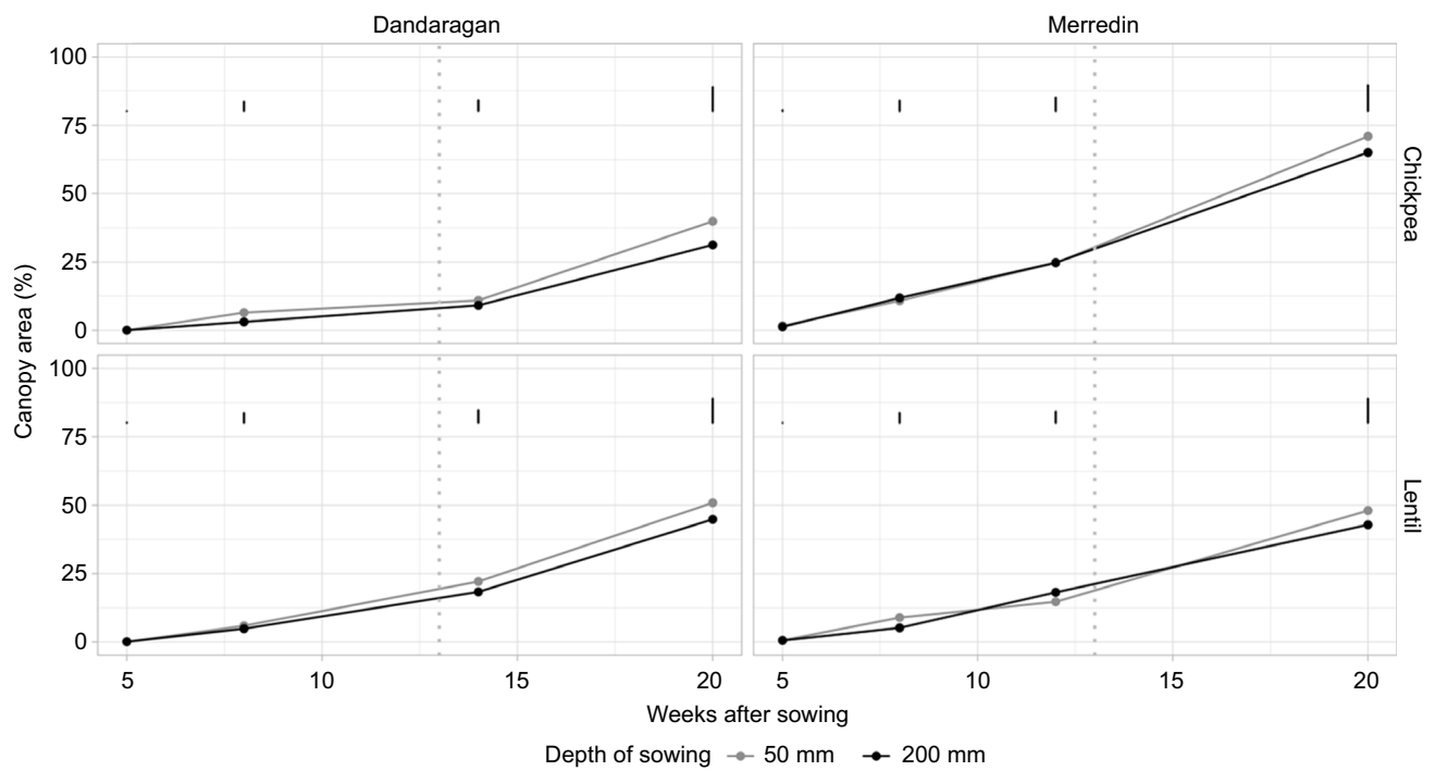
Fig. 7. Canopy development of Striker chickpea and Bolt lentil from standard (50 mm) and deep (200 mm) sowing depths measured as canopy cover over the first 20 weeks after sowing. Dashed line indicates flowering time (50% plot flowering). Canopy cover was measured by counting green pixels in digital images using Canopeo within Matlab. Images are from plots sown in May at Dandaragan and Merredin in Western Australia. Vertical lines represent l.s.d. ( P = 0.05 ) values comparing sowing depths at individual measurement times.
