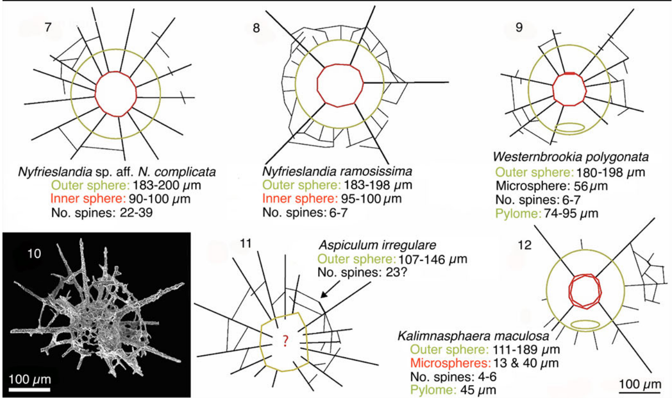
Figure 7. Compilation of μ-CT models, SEM images, and line drawings illustrating the family Aspiculidae from sample PD13. (1, 4, 7) Nyfrieslandia sp. aff. N. complicata ; (2, 5, 8) Nyfrieslandia ramosissima n. sp.; (3, 6, 9) Westernbrookia polygonata n. sp.; (10, 11) Aspiculum irregulare n. sp.; (12) line drawing of Upper Ordovician Kalimnasphaera maculosa after Webby and Blom (1986).
